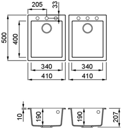
Technical Drawing
