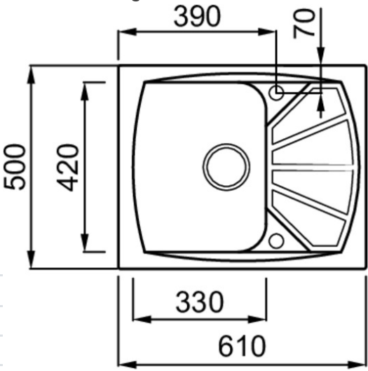
Technical Drawing
